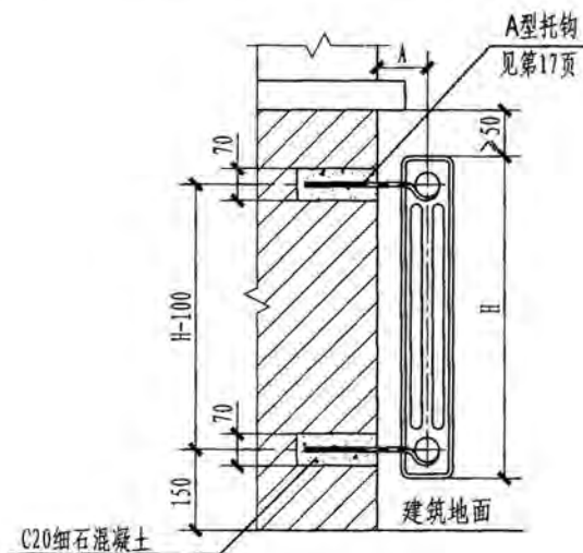
砖墙上安装(I)
